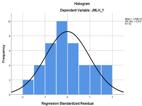
Gambar 2. Histogram
